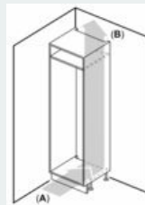
A: Air inlet ≥ 200 cm 2 . Ventilation options B: Air outlet ≥ 200 cm 2 . Ventilation options
