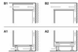
A: Air inlet ≥ 200 cm 2 . Ventilation options B: Air outlet ≥ 200 cm 2 . Ventilation options
